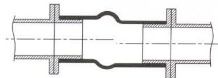
LATERAL DEFLECTION
