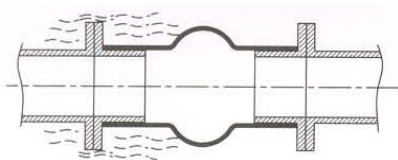
VIBRATION ISOLATION
